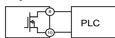
Digital output on terminal 8-9-10 in digital output configuration
